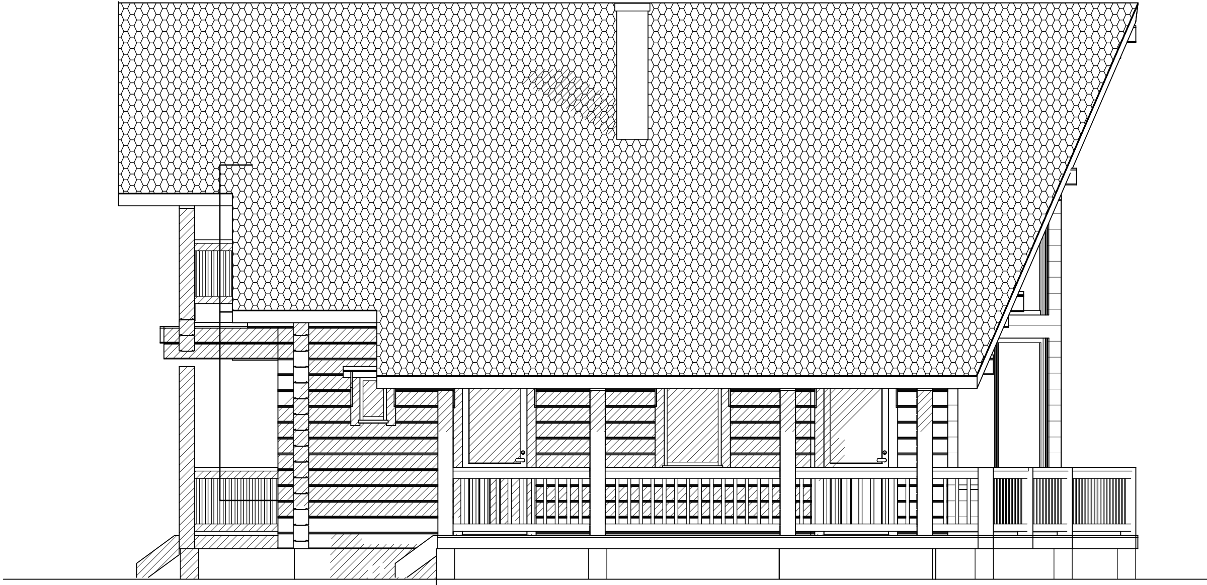
ELEVATIONS 1;50 PROJECT H2-107
